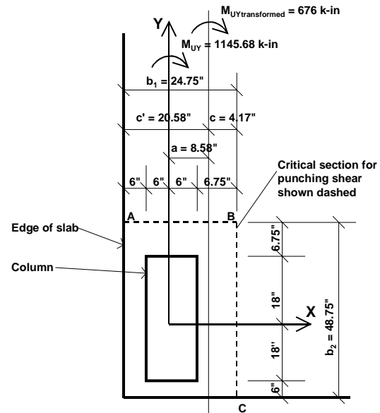
Figure 16: Corner Column, Point 5 in SAFE Model Bending About Y-Axis
