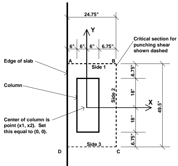
Figure 7: Edge Column With Edge Parallel To Y-Axis, Point 9 in SAFE Model
