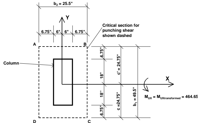
Figure 9: Interior Column, Point 10 in SAFE Model Bending About X-Axis
